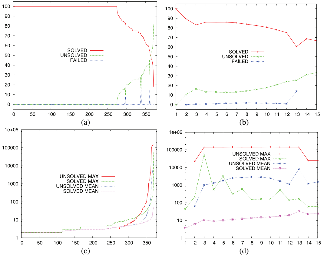
Figure 3: Coverage (a,b) and state evaluations (c,d) data, plotted over individual kinds of BOs (a,c) and |G| (b,d). “SOLVED”: plan found. “UNSOLVED”: search space (with helpful actions pruning) exhausted. “FAILED”: out of time or memory.
