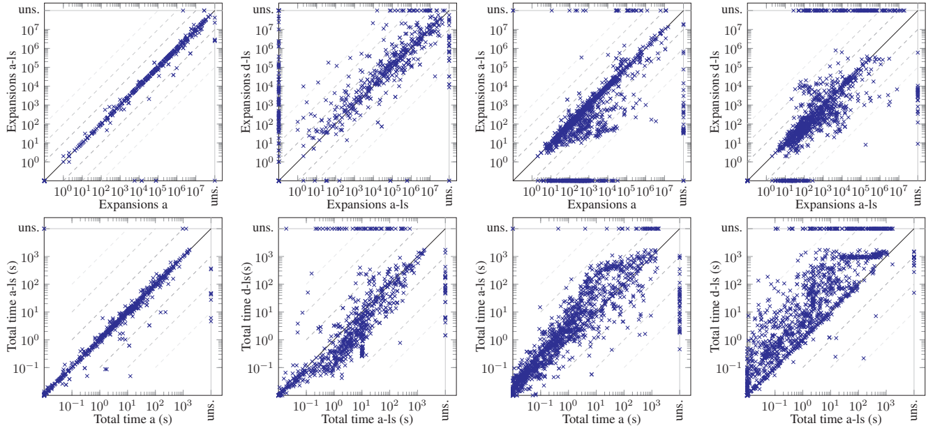
Figure 3: Expansions until last f -layer and total time of a vs. a-ls (left) and a-ls vs. d-ls (right) for A^* with M&S (left block) and lazy greedy search with h^{\text{FF}} and preferred operators (right block).
